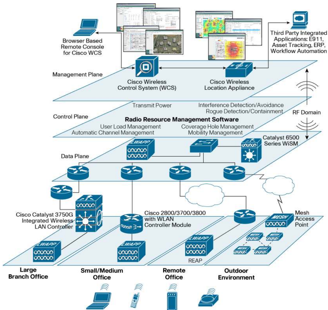
Figure 3. Unified Access Point Deployment
