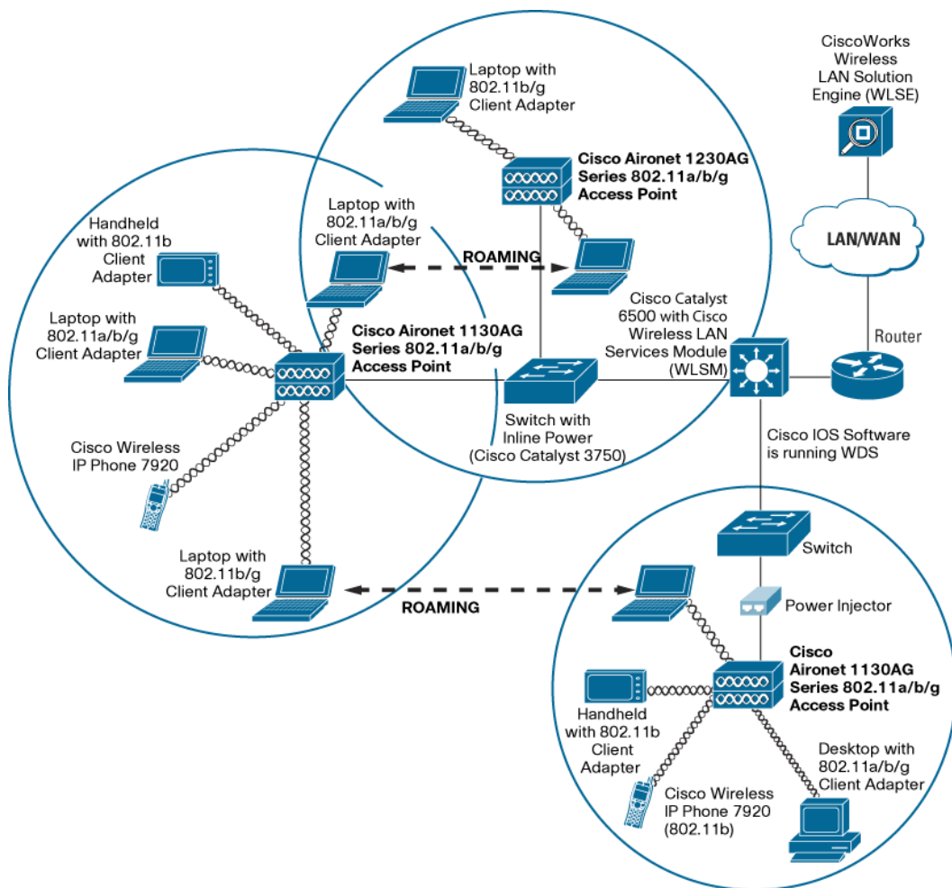
Figure 4. Autonomous Access Point Deployment
