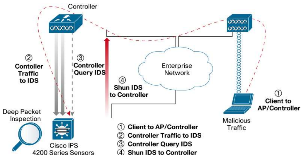
Figure 1. Cisco Unified IDS/IPS Detects Malicious Attacks Allowing the WLAN Controller to Disassociate the Offending Client Device
